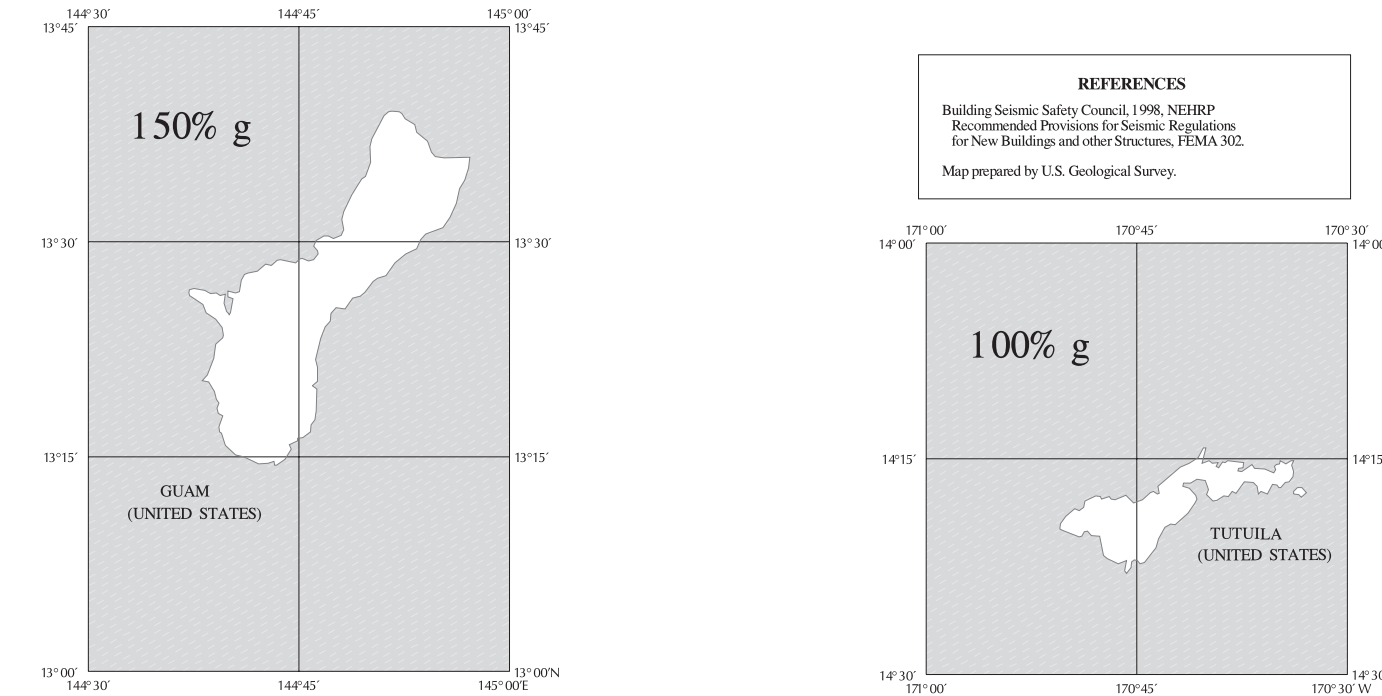
0.2 SEC SPECTRAL RESPONSE ACCELERATION (5% OF CRITICAL DAMPING)
